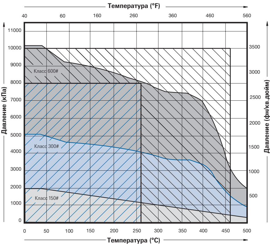
Pressure/Temperature Graph
