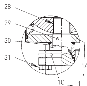
LOWER SHAFT FOR DN 150
