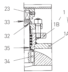
STEM GUIDE DESIGN FOR DN 150
