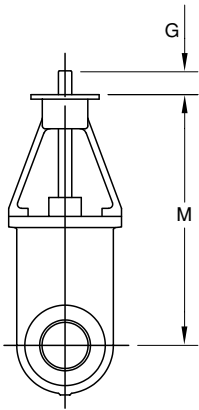
Dimensions and weights ASME Cl. 900
