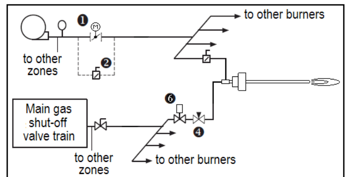
Figure 3.3. Gas Pulse Control. Constant Air
