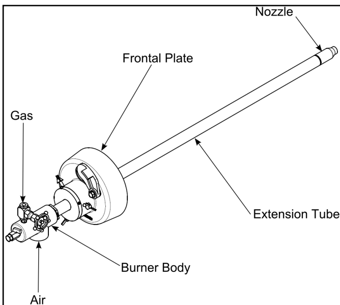
Figure 1.1. ExtensoHeat Burner
