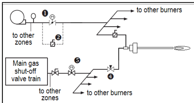
Figure 3.2. Modulating Gas Control. Constant Air
